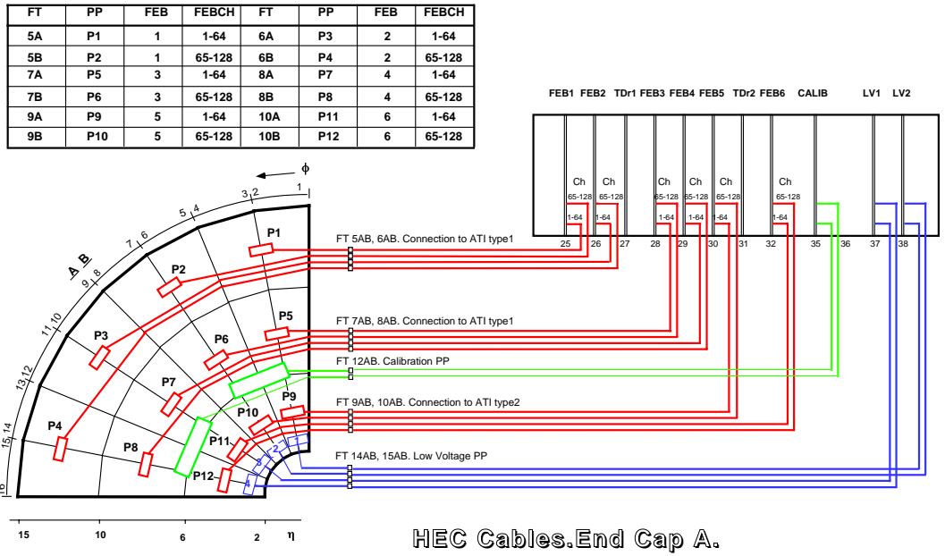
Figure 54: Overview of the signal, LV and calibration cabling for one quadrant of endcap A. Shown are the lines from the patch panels at the rear plane of HEC2 up to FEB boards, including the feed-through connector assignment.
