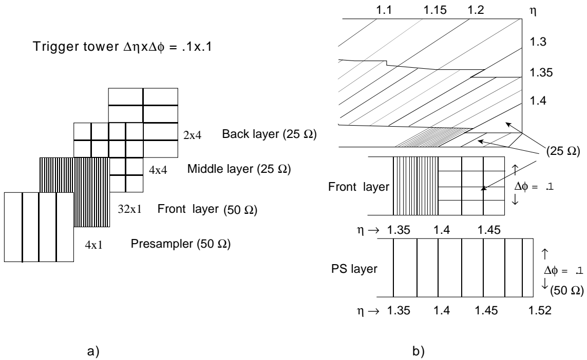
Figure 2: a) Granularity within a trigger tower of the EM barrel ( |\eta| < 1.4 ). There are 64 such trigger towers in azimuth and 2 x 14 in rapidity. b) Granularity at the end of the barrel ( |\eta| > 1.4 ) in r - \eta and r - \phi views.
