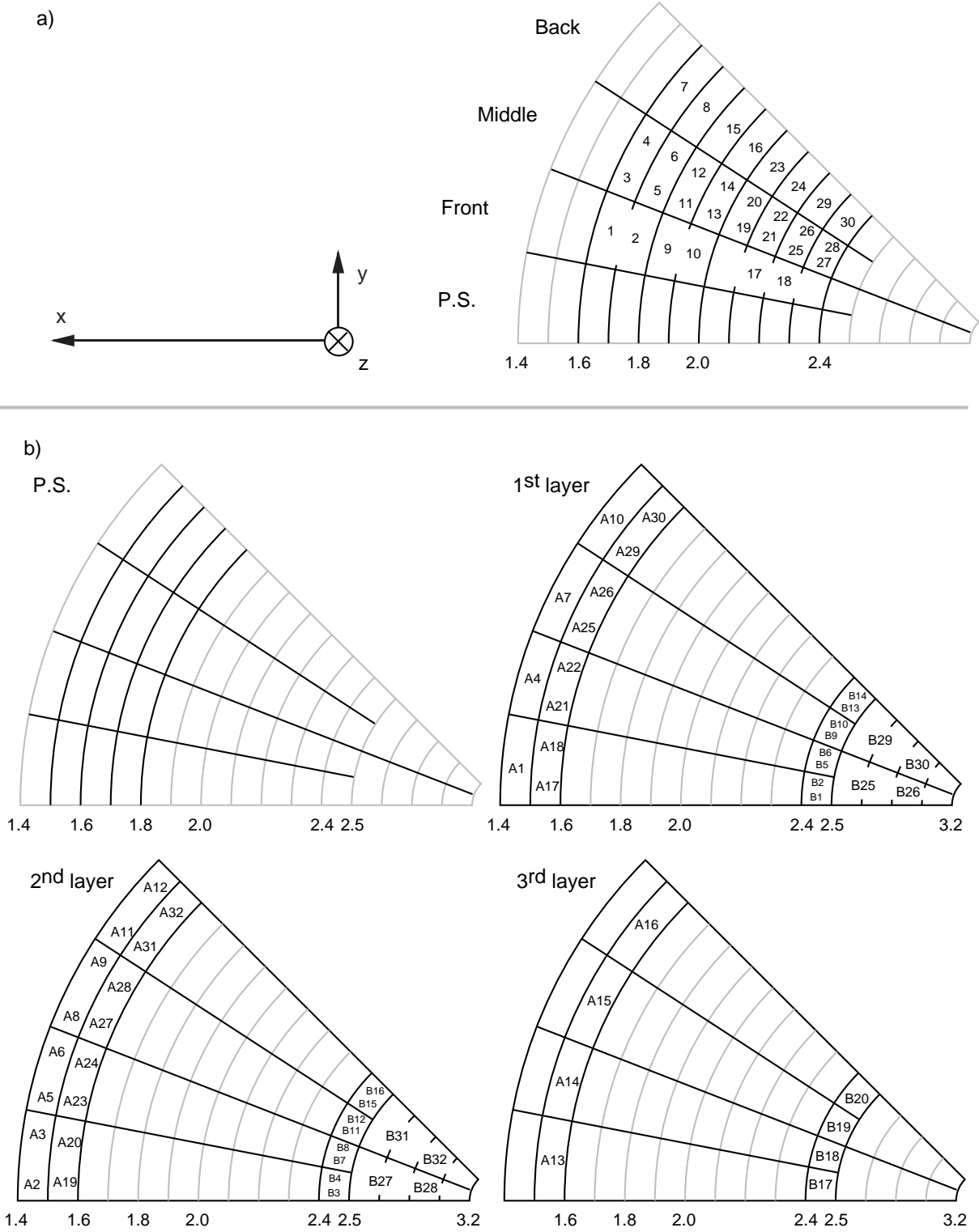
Figure 32: Schematic representation of an EM end-cap wedge ( \Delta\phi = 0.8 ). Concentric lines are drawn at trigger tower boundaries. Calibration harnesses end in 32 low profile connectors numbered 1 to 32. a) Two calibration boards (i.e. 4 calibration harnesses) pulse the “standard” region. The first harness is cabled to the region 0 < \phi < 0.2 , the second to 0.2 < \phi < .4 and so on. Otherwise their cabling is identical and defined by a). b) One calibration board pulse the “special” region of an EM end-cap wedge: \Delta\phi = 0.8 . The cabling to the detector is defined by b).
