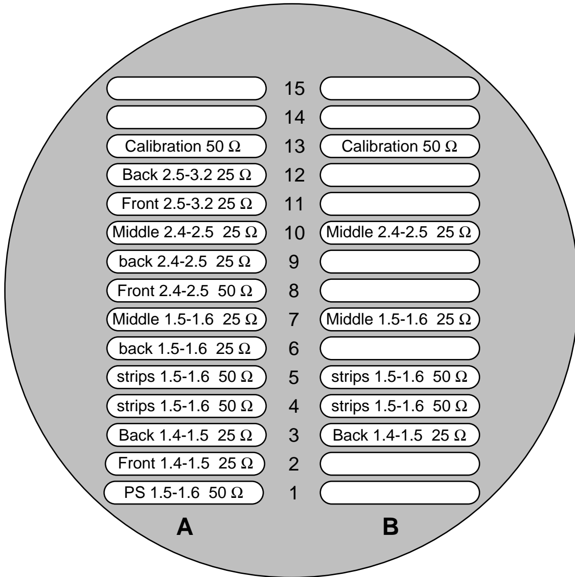
Figure 38: Map of the flange seen from liquid argon for the “special” feedthrough of the NA31 cryostat. The cable impedance (50 or 25Ω) together with a calorimeter zone or a function is indicated for each connector.
