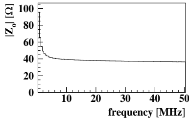
Figure 4: Characteristic impedance measured as a function of frequency.
