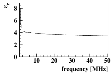
Figure 8: Relative dielectric constant as a function of frequency.
