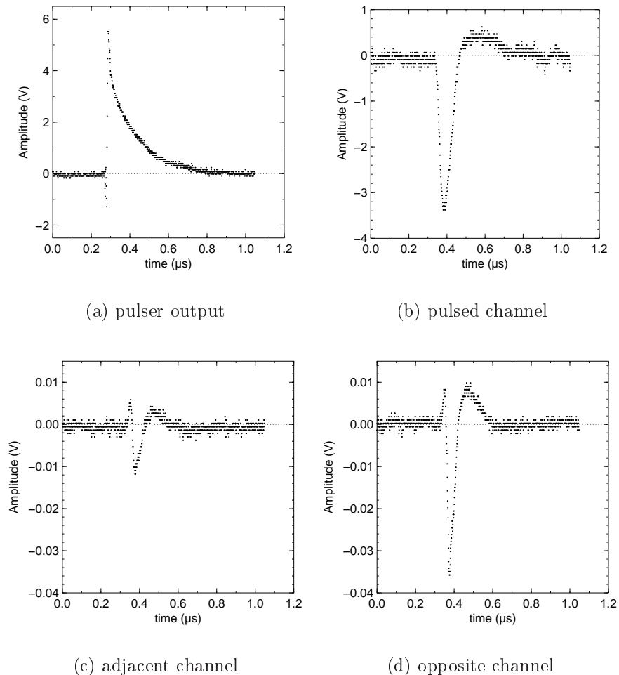
Figure 13: A sample signal from the pulser output before amplification and shaping is shown in (a), and after amplification and shaping in (b). Signals from an adjacent and opposite neighbor after amplification and shaping are shown in (c) and (d) respectively.
