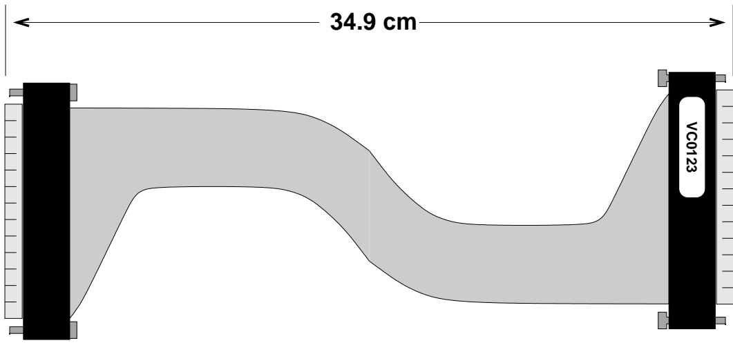
Figure 2: A schematic of an endcap signal feedthrough vacuum cable.
