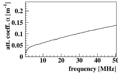
Figure 5: Attenuation coefficient measured as a function of frequency.
